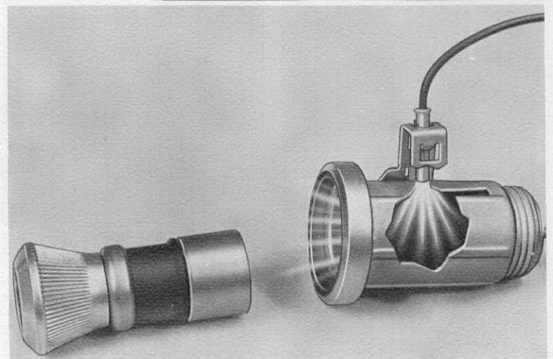
The illumination of the cigar lighter housing, as illustrated here, will be featured on 1967 Pontiacs. When limited space will not permit the use of the conventional bulb and socket, SeeLite may sometimes be the only way possible to light an instrument panel component.
