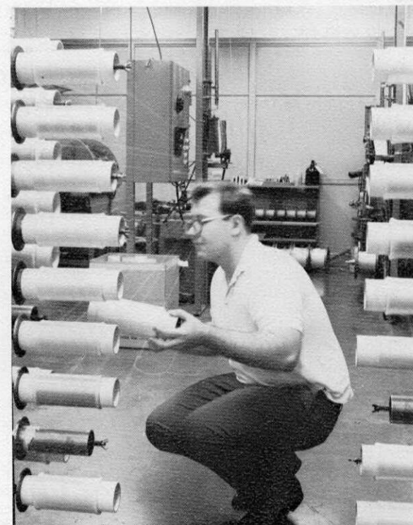
William Teglas changes a supply tube of impregnated fiber glass in the parallel stranding operation.
